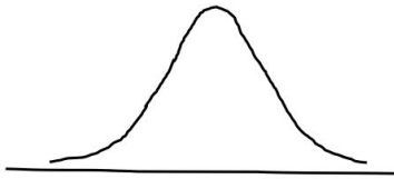
Normal Distribution
